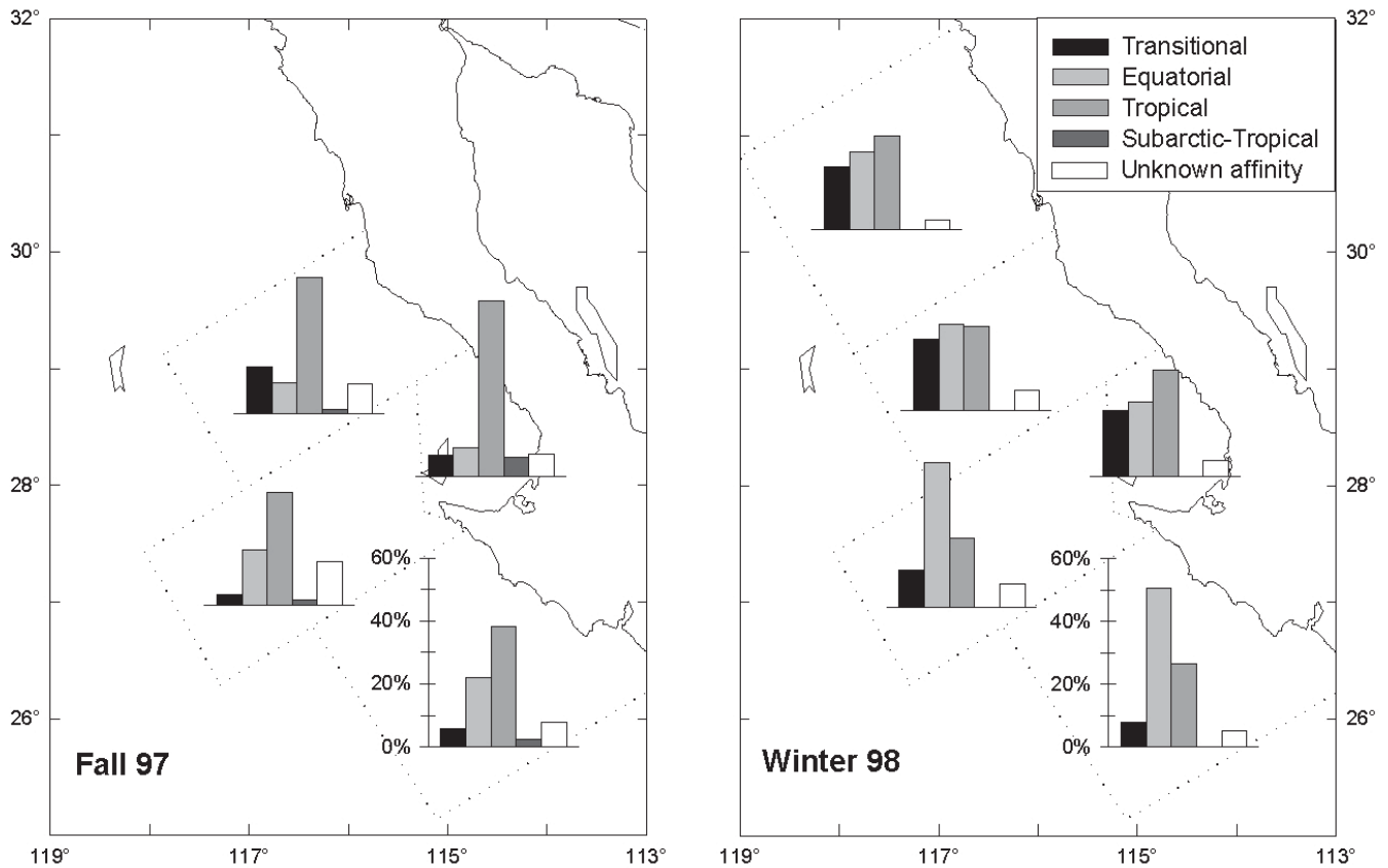
Fig. 4. Mean relative abundance by biogeographic groups of dominant copepod species by areas during Fall 97 and Winter 98.
