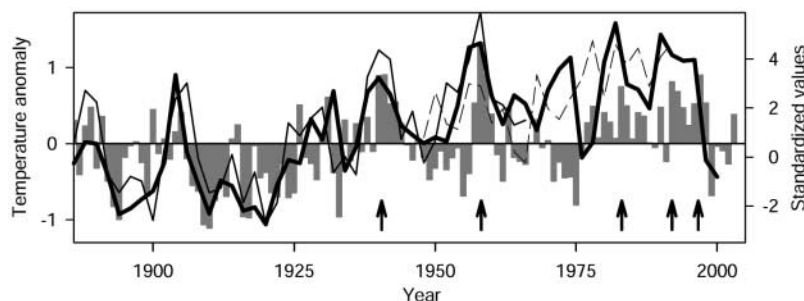
Fig. 3. Comparison of PC1 (bold solid line) with the SST record from the updated Kaplan reconstruction for the 5^{\circ} \times 5^{\circ} grid centered at 122.5^{\circ}\text{W} , 32.5^{\circ}\text{N} (vertical bars) in the California Current near the SBB. PC1 is correlated with variations in SST from comparable 2-year averages of SSTs ( r^2 = 0.33 ; P < 0.001 ). Arrows indicate strong El Niño events in the California Current. Also shown is the agreement of foraminiferal variations from PC1 (core BC3001) with those from two other cores in the SBB. Thin dashed line illustrates variations in averaged abundance of the same species loaded on PC1 from a core taken in 1992 and analyzed in this study. Thin solid line illustrates average of the principal species loaded on PC1 ( G. bulloides , N. dutertrei , G. ruber , O. universa , and the combination of G. calida and G. siphonifera ) from a core taken in 1969 and analyzed by A. Soutar and W. Berger.
